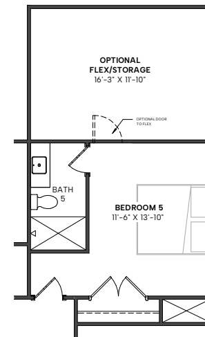
BEDROOM 5 W/ FULL BATH + FLEX/STORAGE ROOM ILO FLEX ROOM +205 SQ FT
