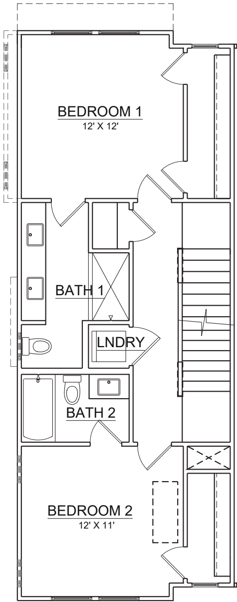
THIRD FLOOR
