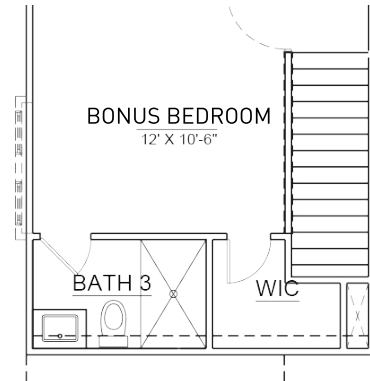
OPT. FULL BATHROOM IN BONUS BEDROOM
